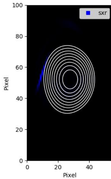
#92292 Profile @ 52013ms
