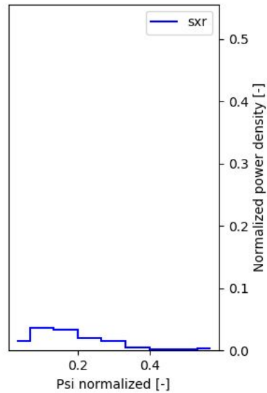
#92292 Profile @ 52013ms
